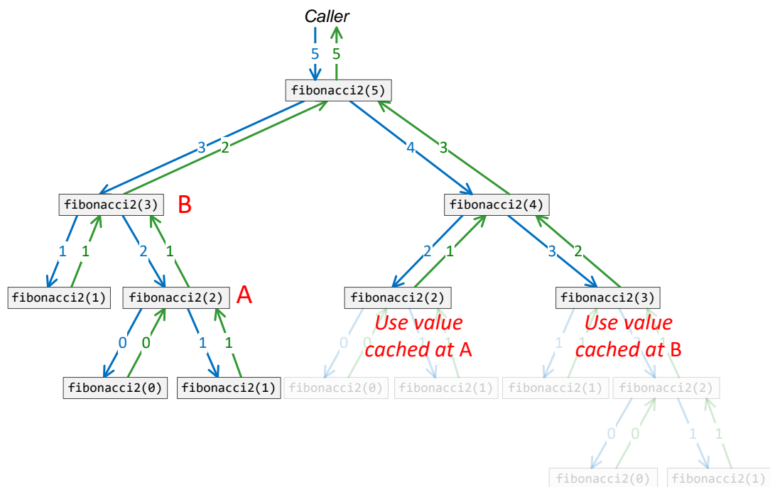
Figure 21.1 The hierarchy of recursive function calls that result from the call fibonacci2(5) . Note that the calls of fibonacci(2) and fibonacci(3) on the right side of the tree need no recursive calls; this is because their earlier calls on the left side of the tree stored their results in the map for instant retrieval.
