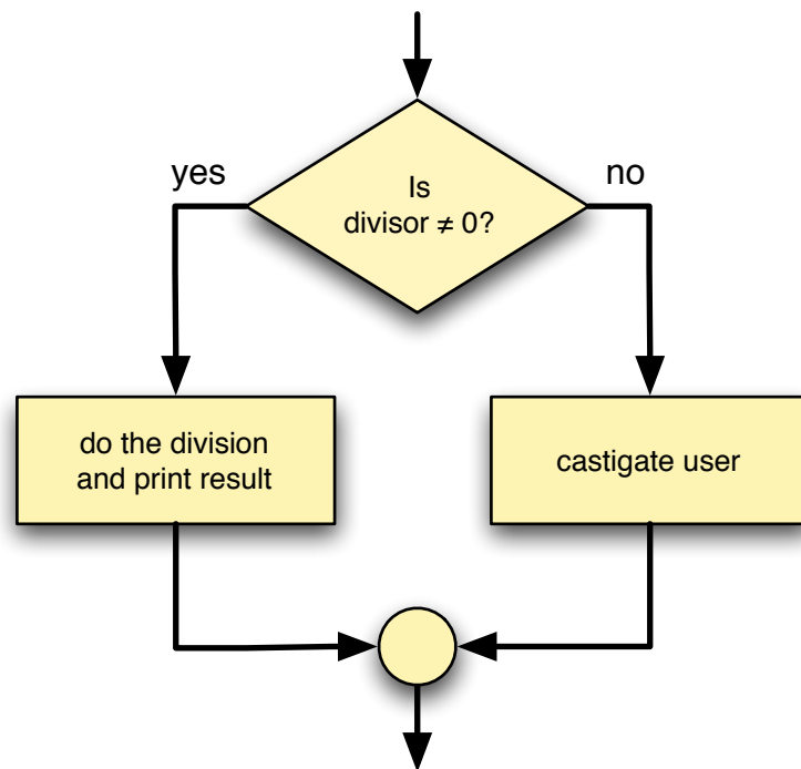
Figure 5.2 if/else flowchart
